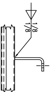
WELDMENT DETAIL -B-
